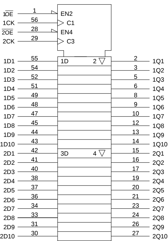
IEC Logic Symbol
