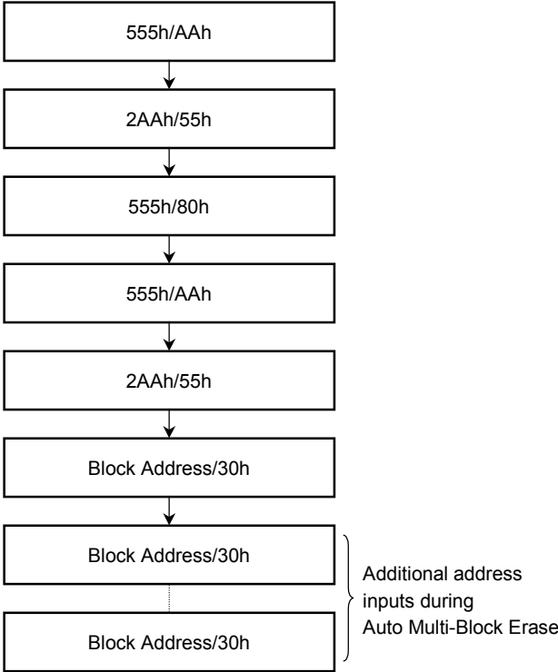
Auto Block/Auto Multi-Block Erase Command Sequence (address/data)
