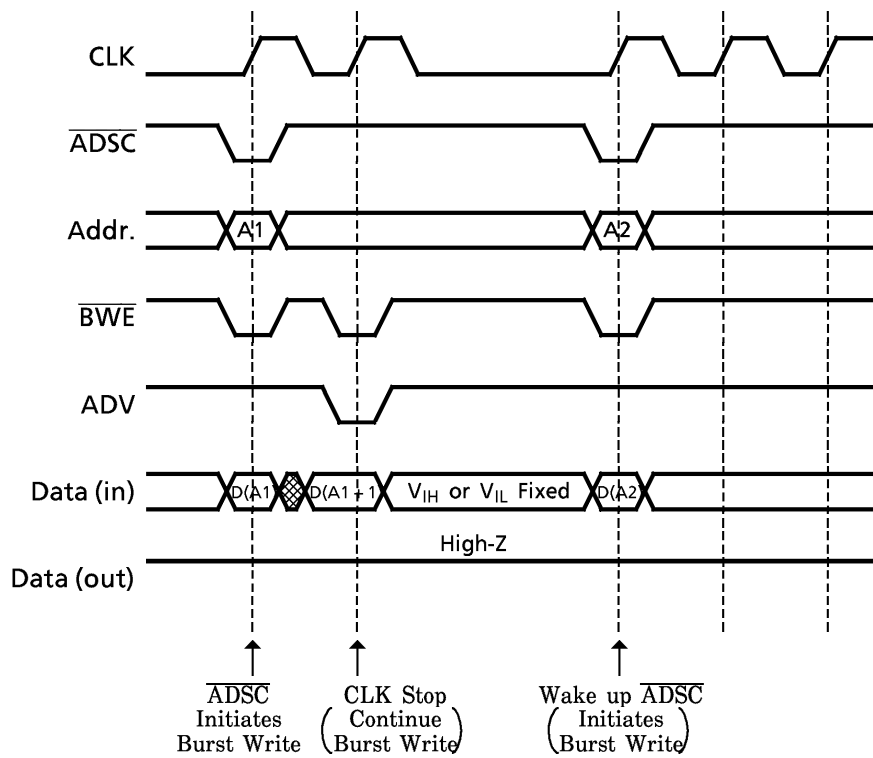
ii) Stop-Clock Timing for Write Operation
