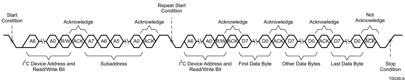
Figure 29. Multiple-Byte Read Transfer
