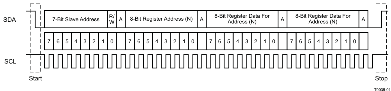
Figure 25. Typical I 2 C Sequence
