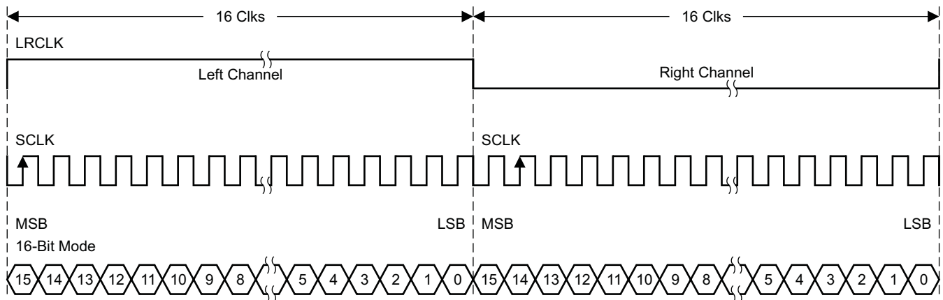
Figure 21. Left-Justified 32- f_s Format
