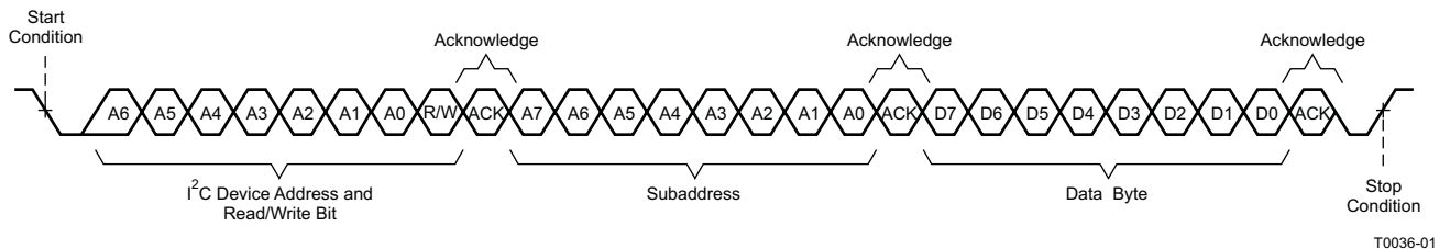
Figure 26. Single-Byte Write Transfer
