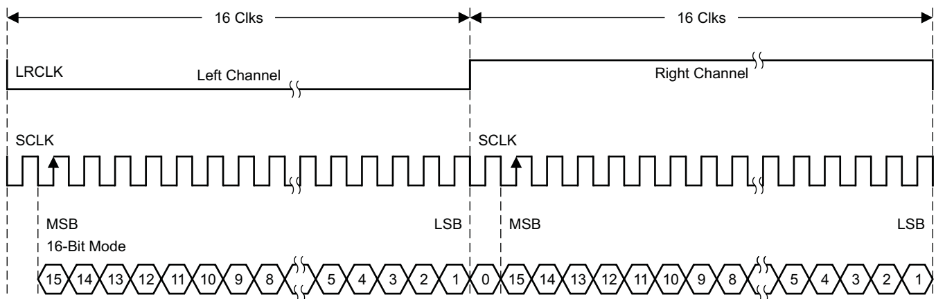
Figure 18. I 2 S 32-f s Format
