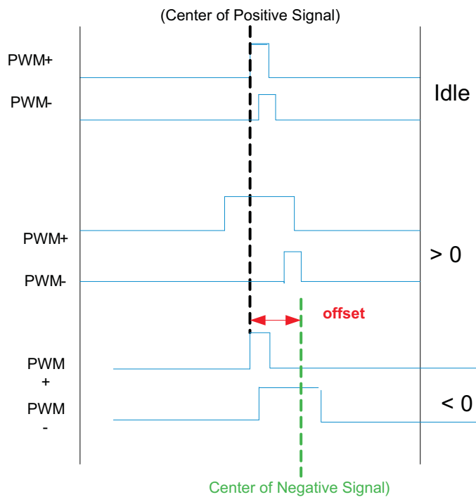
Figure 2-4. Ternary Modulation
