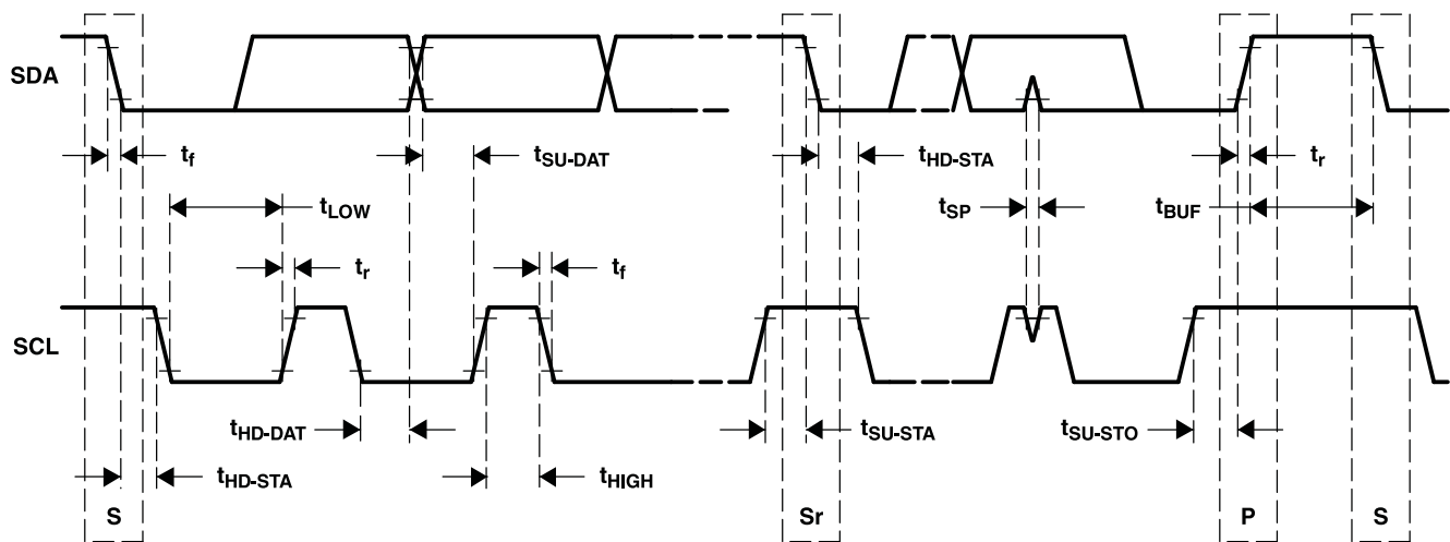
Figure 7-2. SCL and SDA Timing
