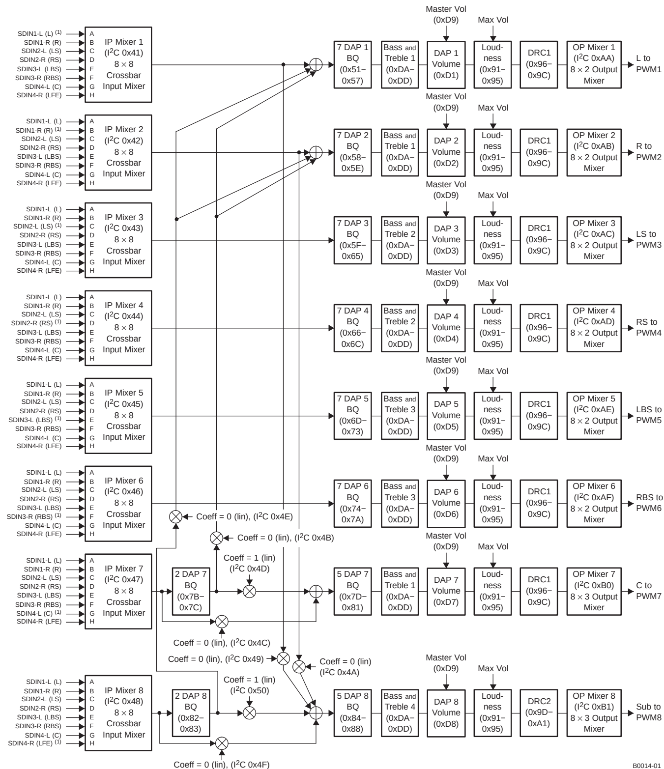
Figure 2-1. TAS5508C DAP Architecture With I²C Registers (Fs ≤ 96 kHz)
