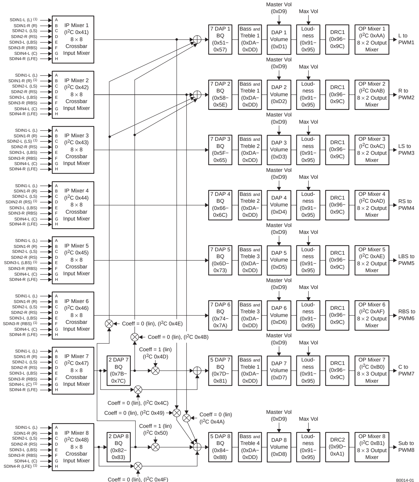
Figure 2-1. TAS5508B DAP Architecture With I²C Registers ( f_s \leq 96 kHz)
