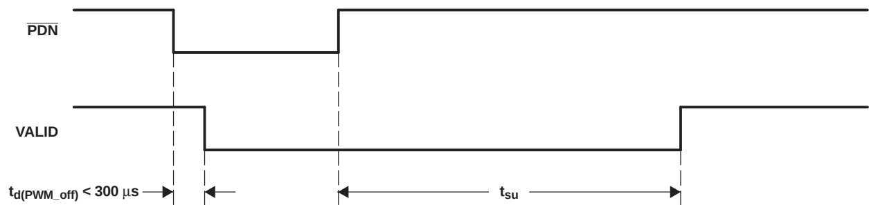
Figure 4-6. Power-Down Timing
