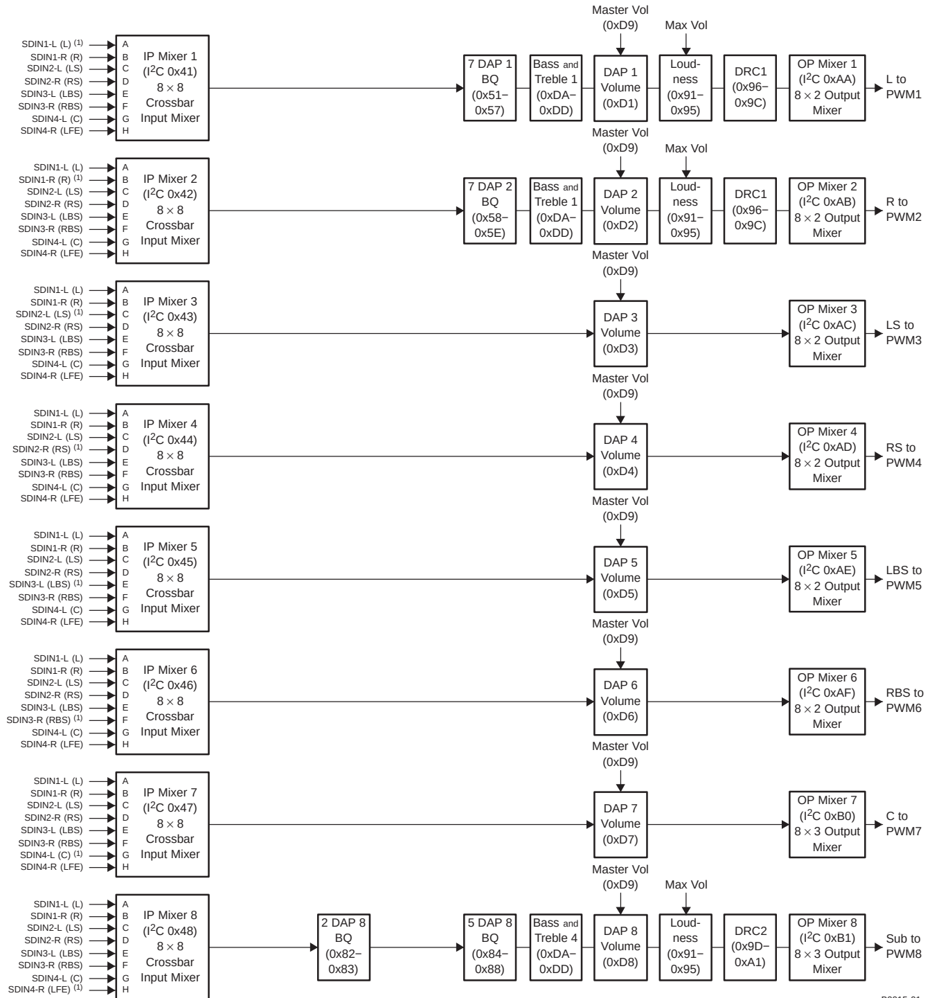
Figure 2-2. TAS5508B Architecture With I²C Registers ( f_s = 176.4 kHz or f_s = 192 kHz)
