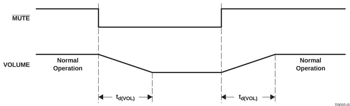
Figure 4-8. Mute Timing
