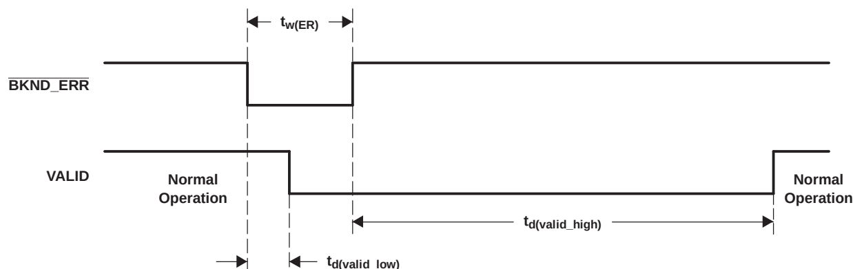
Figure 4-7. Error-Recovery Timing
