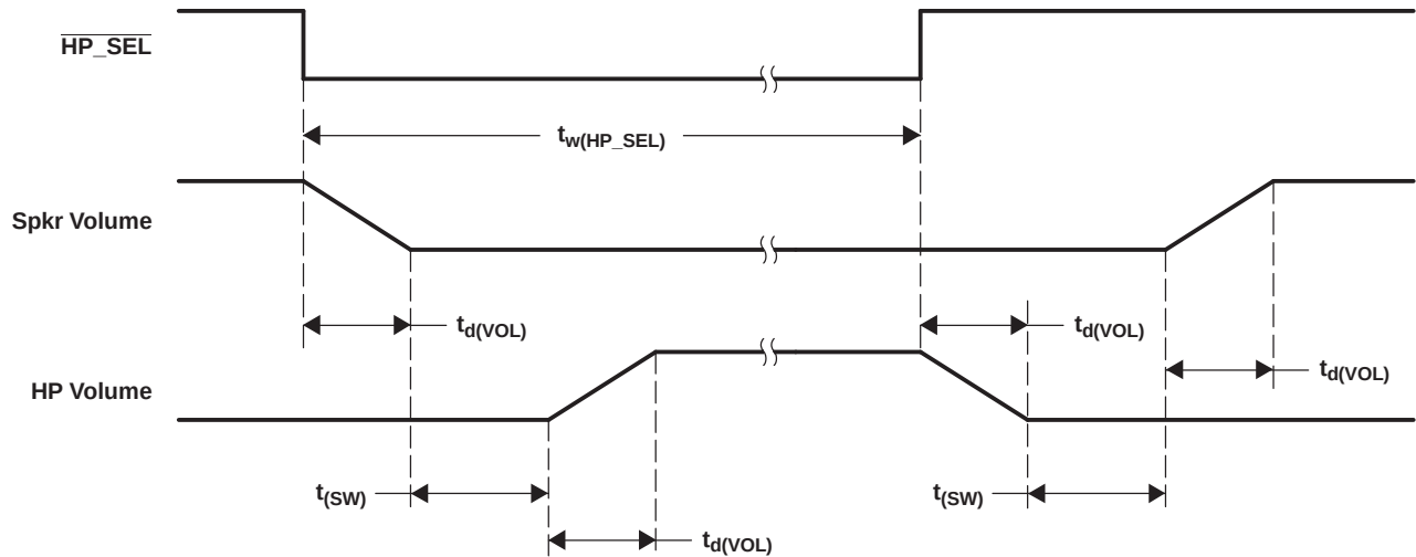
Figure 4-9. \overline{\text{HP\_SEL}} Timing
