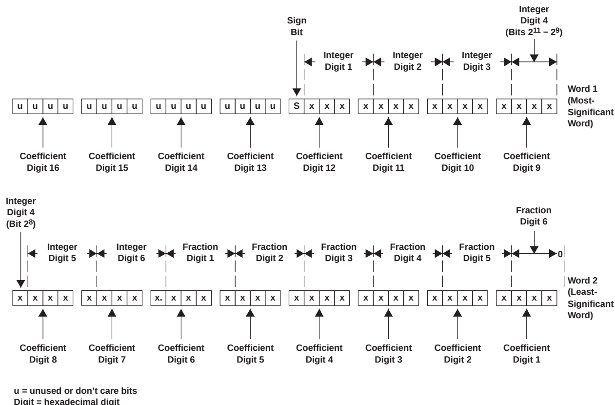
Figure 2-9. Alignment of 25.23 Coefficient in Two 32-Bit I²C Words
