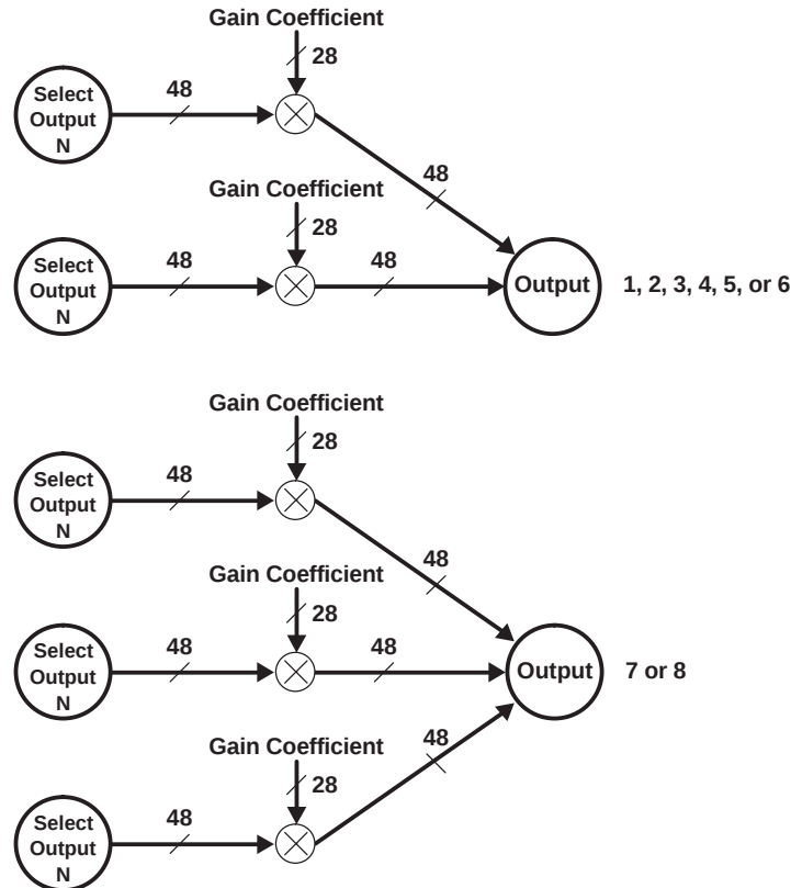
Figure 2-18. Output Mixers
