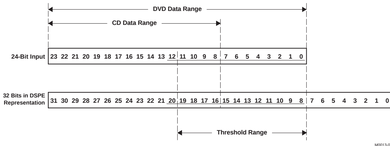
Figure 2-13. Automute Threshold
