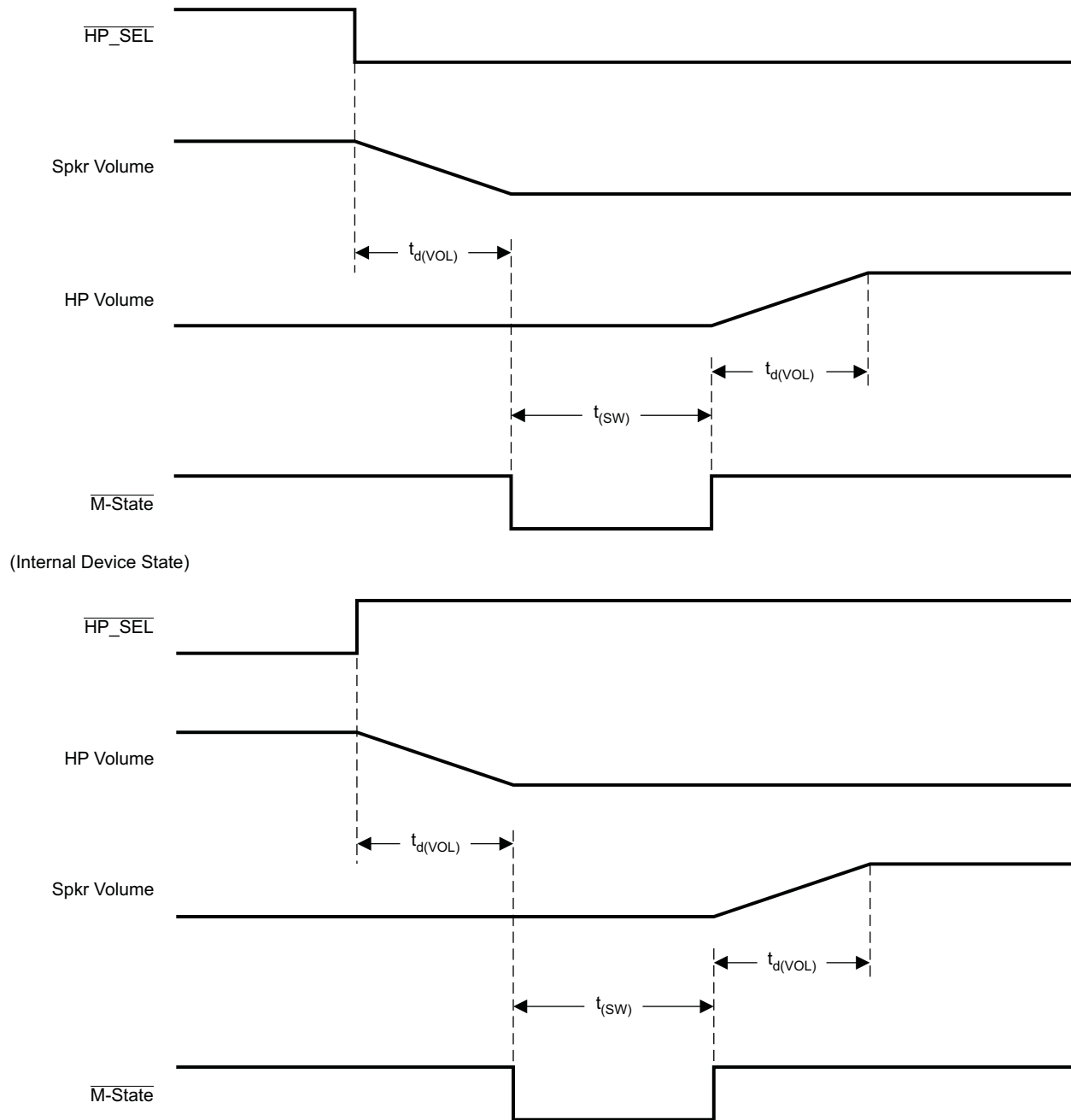
Figure 4-8. \overline{\text{HP\_SEL}} Timing
