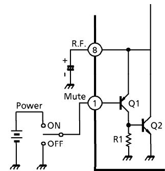
Fig.5 Mute circuit
