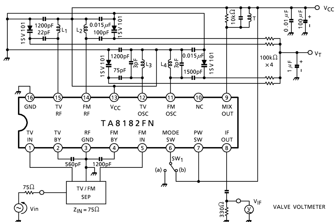
Test Circuit 2
