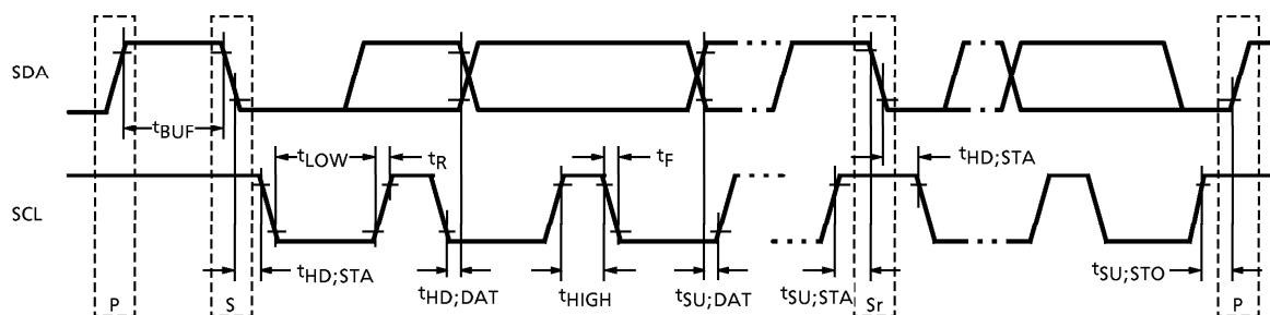
Fig.2 I²C bus data timing chart (Rising edge timing)
