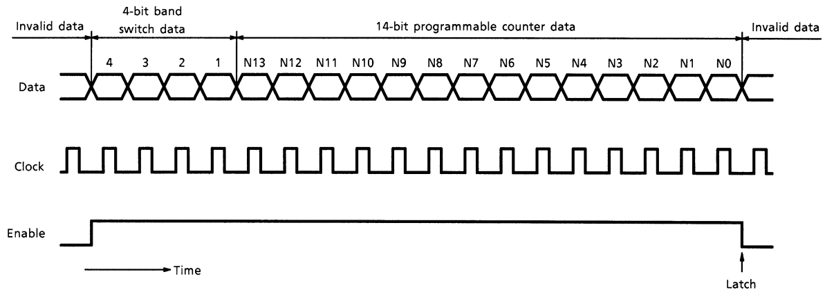
Fig.3 Normal data format (18-bit transmission)
