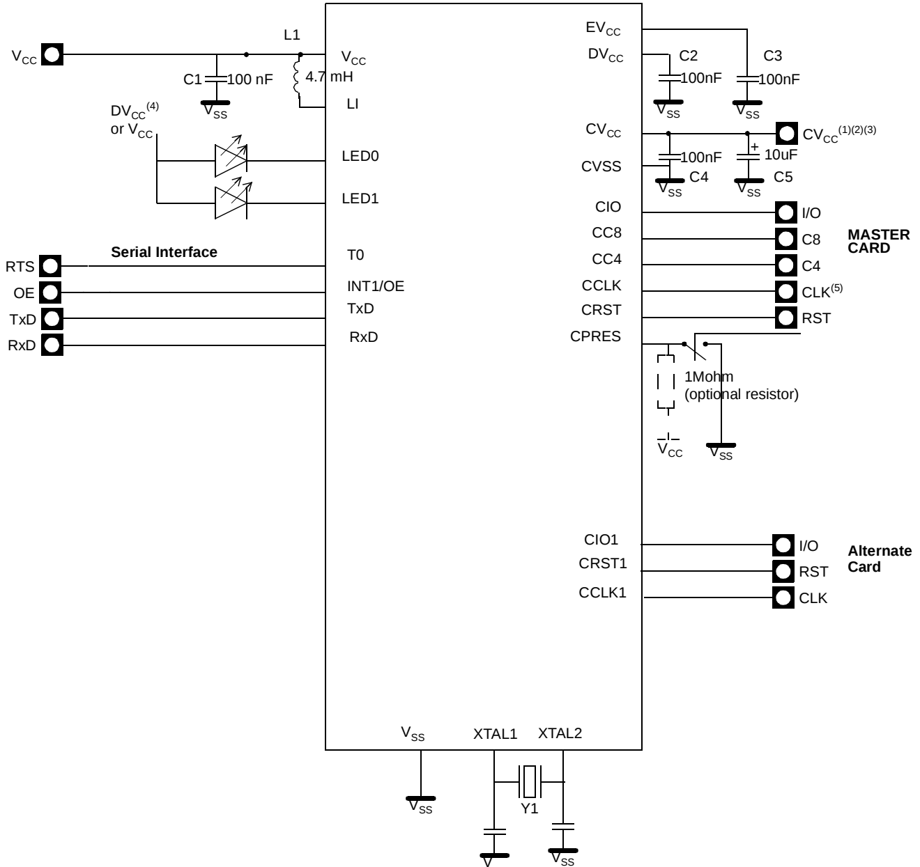
Figure 54. Typical Application Diagram
