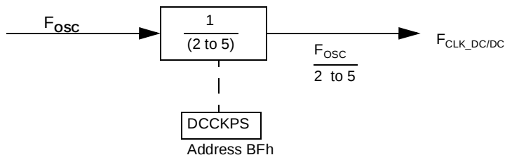
Figure 12. Functional Block Diagram
