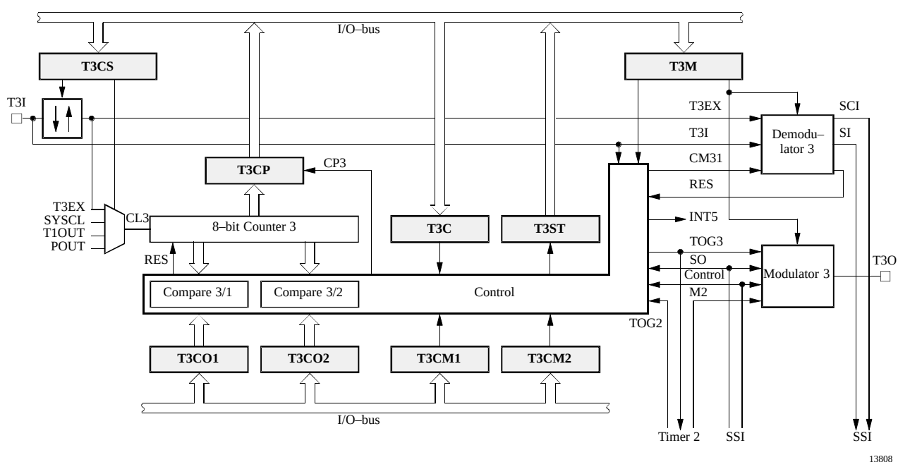
Figure 44. Timer 3
