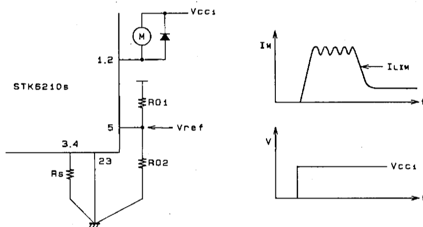
Figure 3 External Peripheral Circuit and Motor Startup Timing Chart
