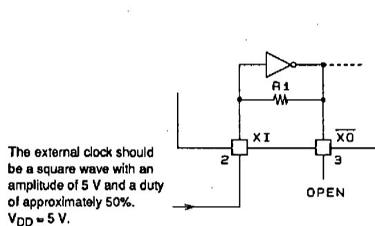
External clock input
