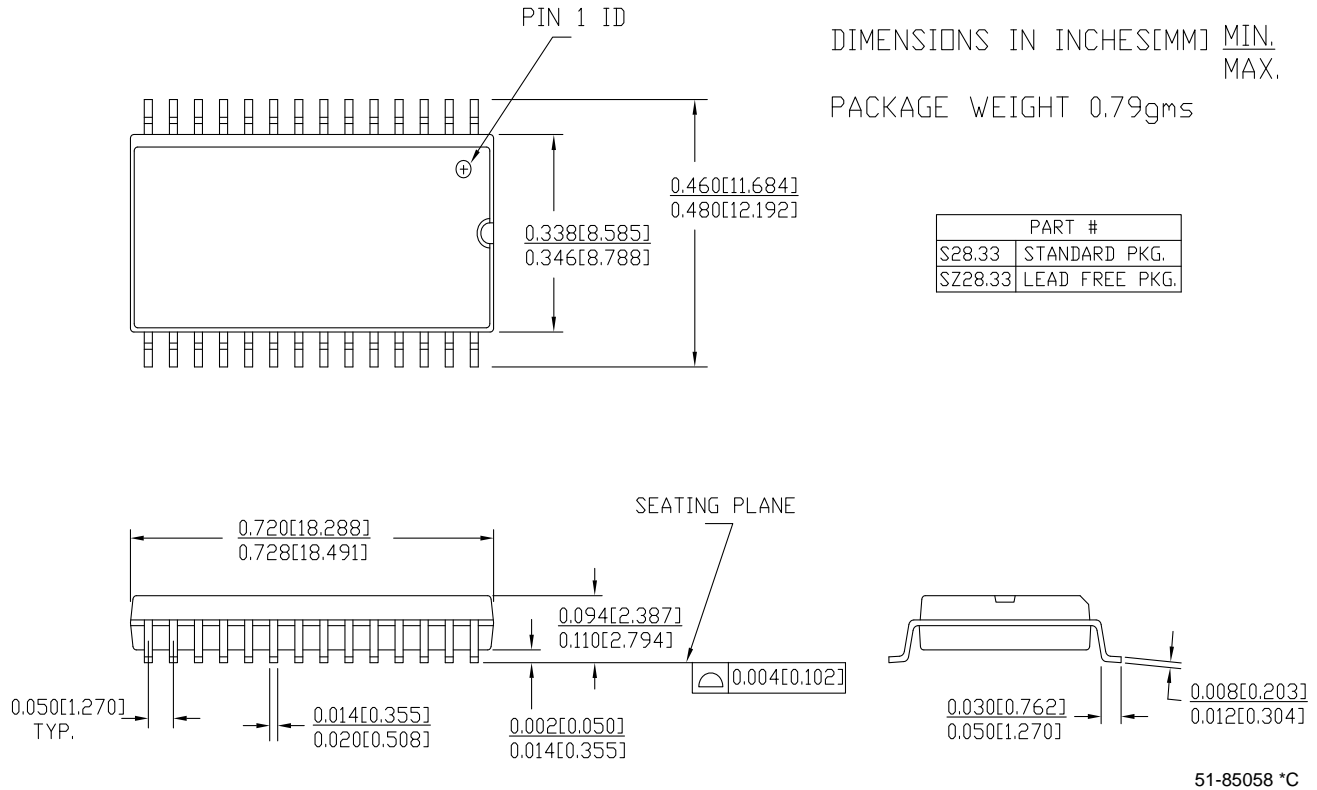
Figure 14. 28-Pin (330 mil) SOIC (51-85058)
