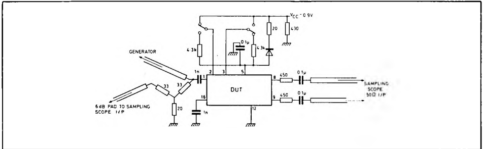
Fig. 3 Test circuit
