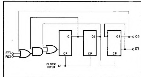
Fig. 2 Logic diagram
