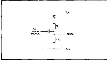
Fig. 6. Recommended input bias configuration for capacitive coupling to a continuous 50 \Omega signal source
