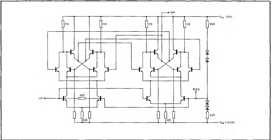
Fig. 3 Circuit diagram of 1st element (I-2) showing input biasing arrangement
