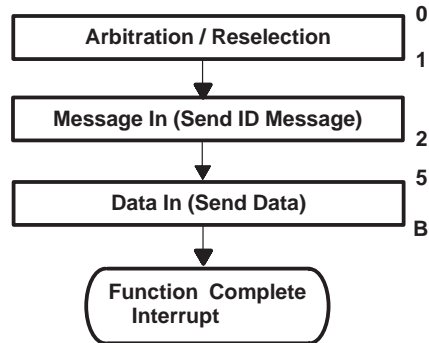
Figure 4–4. Reselect and Send Data (Target)
