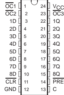
SN74ALS29845 . . . FN Package (Top View)
