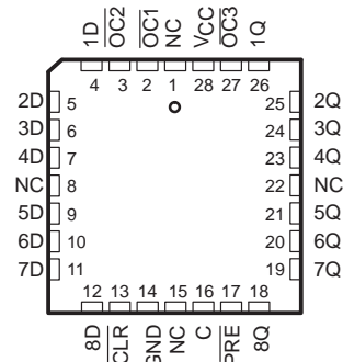
SN74ALS29846 . . . DW or NT Package (Top View)
