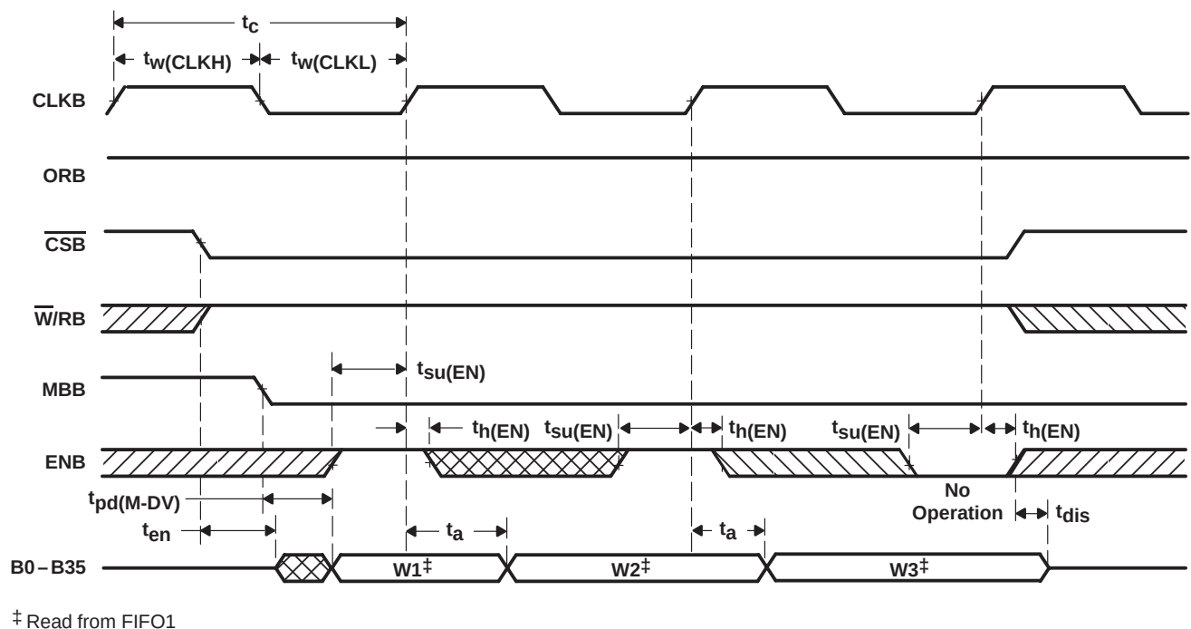
Figure 6. Port-B Read-Cycle Timing for FIFO01
