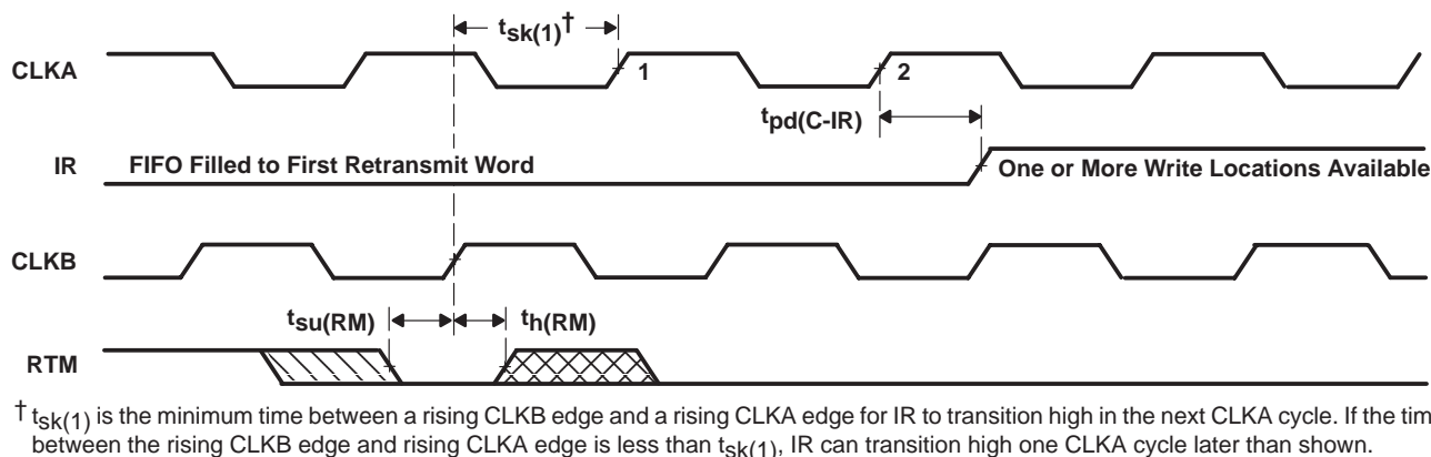
Figure 12. IR Timing From the End of Retransmit Mode When One or More Write Locations Are Available
