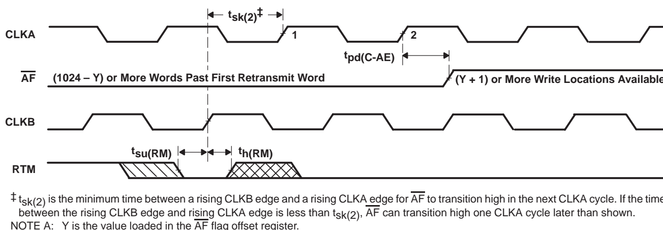
Figure 13. AF Timing From the End of Retransmit Mode When (Y + 1) or More Write Locations Are Available
