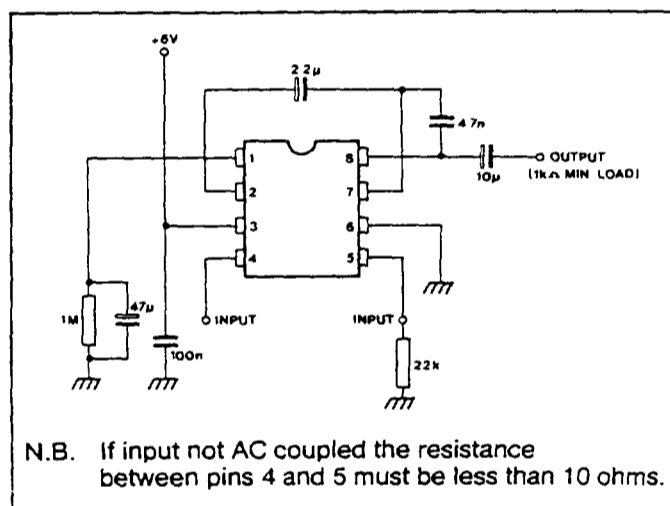
Fig.4 SL6270 test and application circuit
