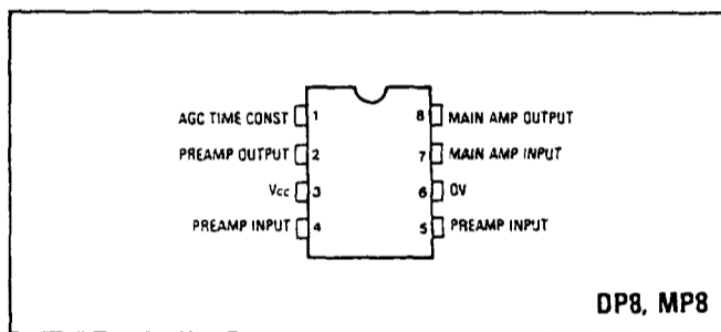
Fig. 2 Pin connections, SL6270 - DP (top view)
