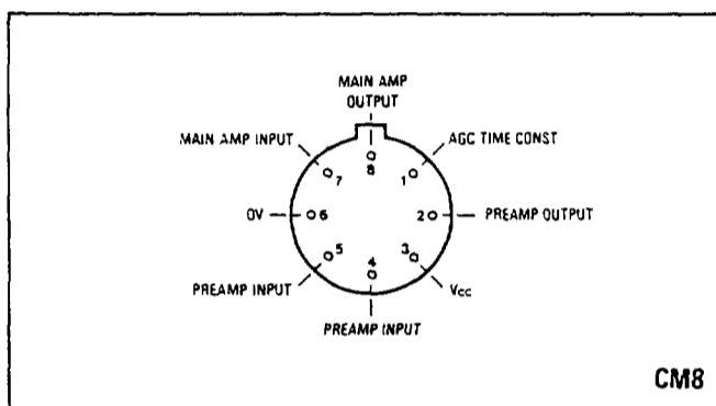
Fig. 1 Pin connections, SL6270 - CM (bottom view)
