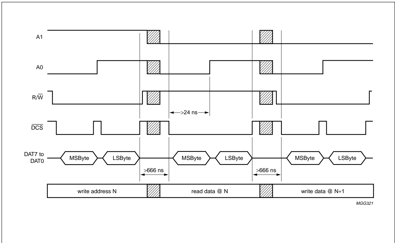
The descrambler internal register address is incremented automatically.
