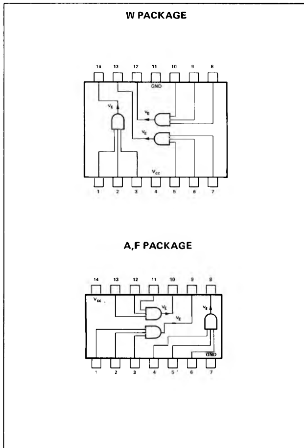
PIN CONFIGURATIONS
