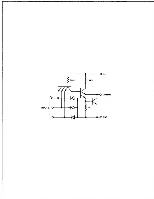
SCHEMATIC (each expander)
