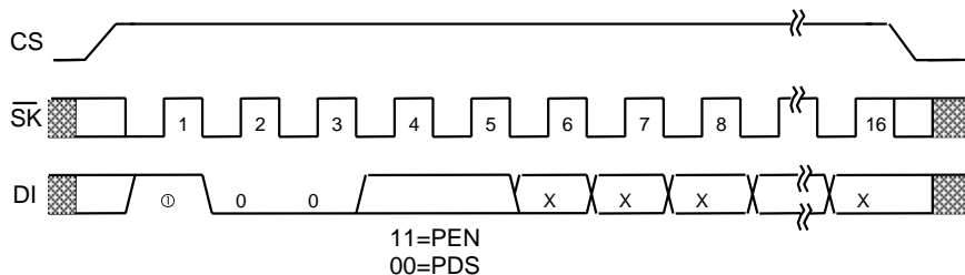
Figure 9 PEN/PDS Timing
