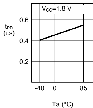
2.7 Data output delay time t_{PD} - Ambient temperature T_a
