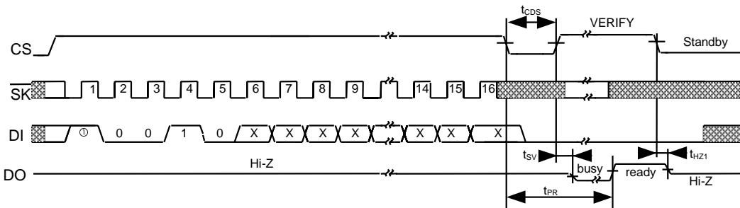
Figure 8 ERAL Timing
