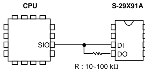
Figure 10 3-wire interface
