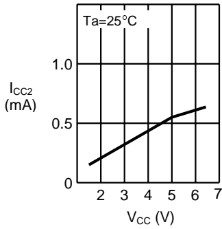
1.9 Current consumption (PROGRAM) I_{CC2} - Power supply voltage V_{CC}
