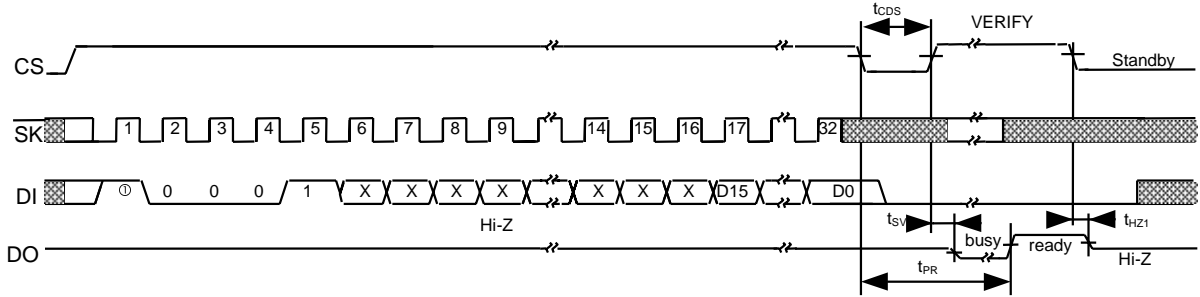
Figure 7 WRAL Timing
