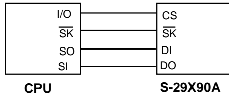
Figure 11 Connectin Example
