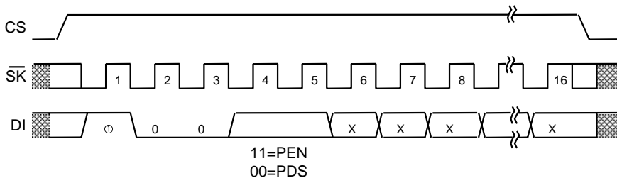
Figure 9 PEN/PDS Timing
