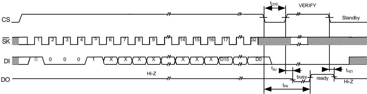
Figure 7 WRAL Timing
