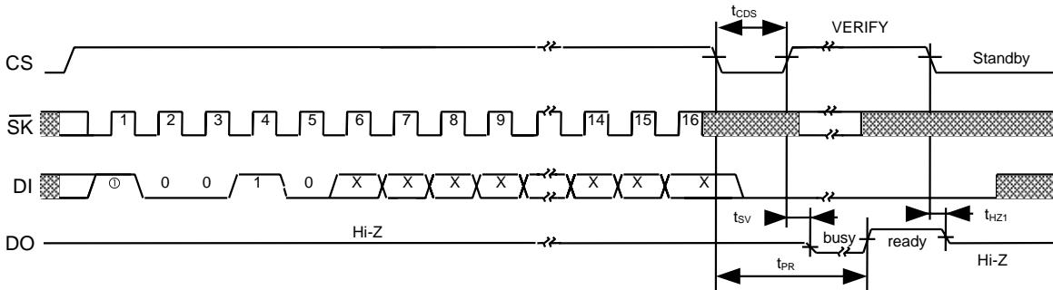
Figure 8 ERAL Timing
