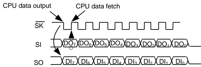
Figure 12 Serial Shift Timing
