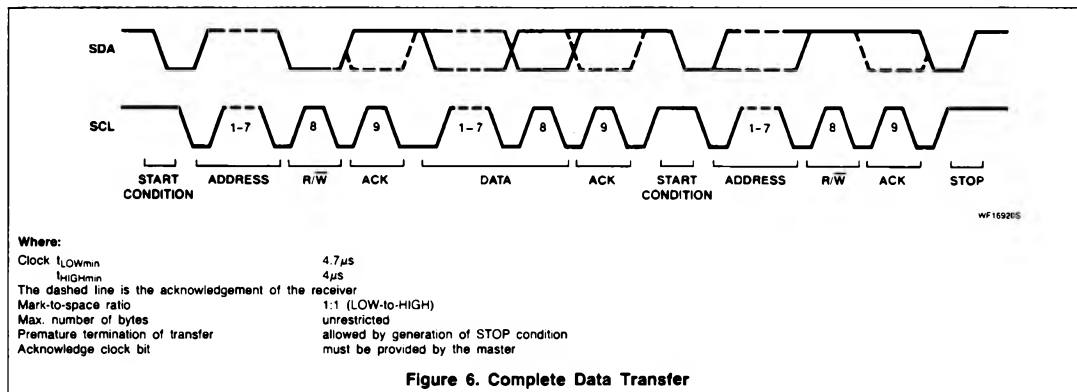
Figure 6. Complete Data Transfer
