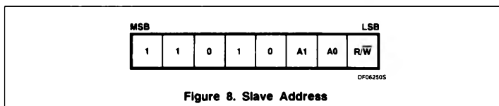
Figure 8. Slave Address
