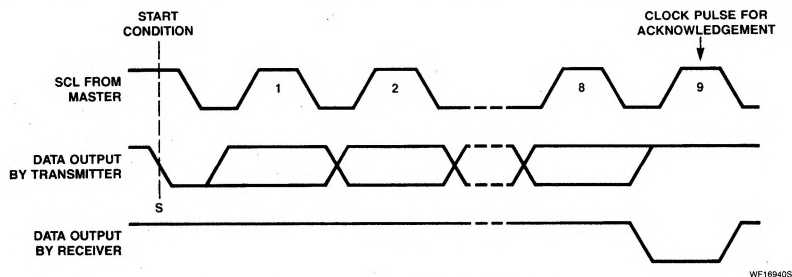
Figure 4. Acknowledgement on the I 2 C Bus
