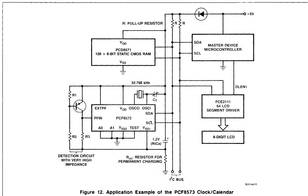
Figure 12. Application Example of the PCF8573 Clock/Calendar
