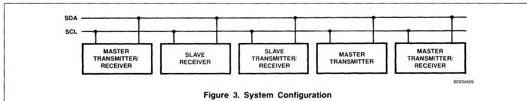
Figure 3. System Configuration
