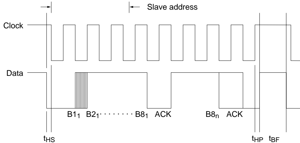
FIGURE 2. I 2 C Bus Timing
