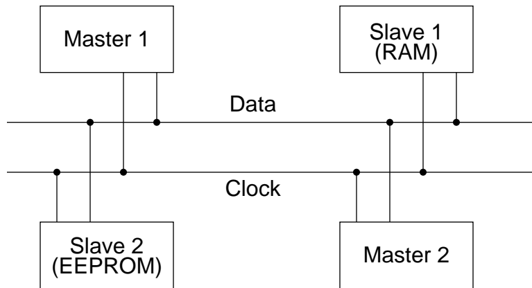
FIGURE 1. I 2 C-Bus Configurations
