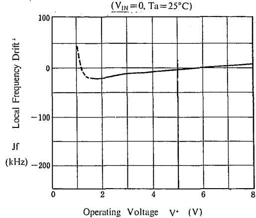
Local Frequency Drift vs. Operating Voltage
