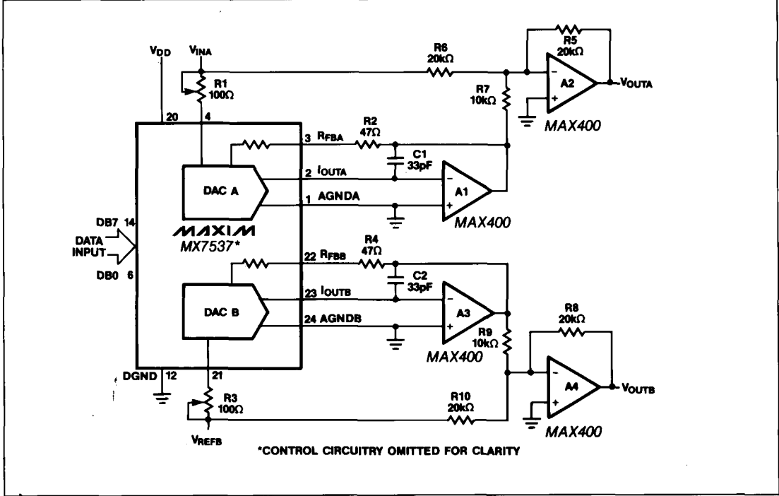
Figure 5A. MX7537 Bipolar Operation (Offset Binary Coding)
