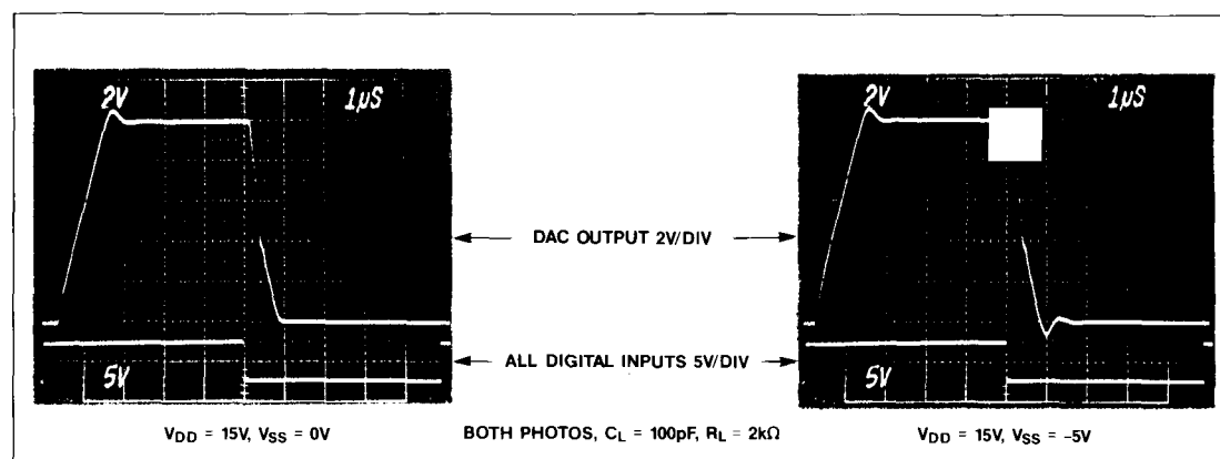
Figure 3. Dynamic Response
