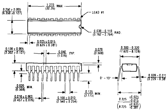
24 Lead Plastic Narrow DIP (NG) \theta_{JA} = 120^{\circ}\text{C/W} \theta_{JC} = 60^{\circ}\text{C/W}
