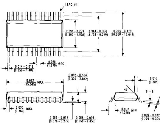
24 Lead Small Outline, Wide (WG) \theta_{JA} = 85^{\circ}\text{C/W} \theta_{JC} = 45^{\circ}\text{C/W}
