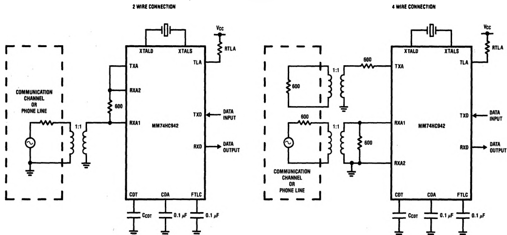
Interface Circuits for MM74HC942 300 Baud Modem
