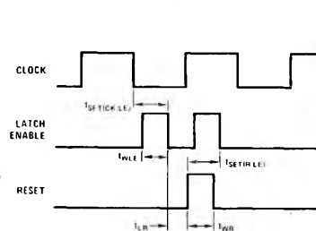
Input Waveforms
