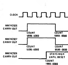
Carry-Out Waveforms
