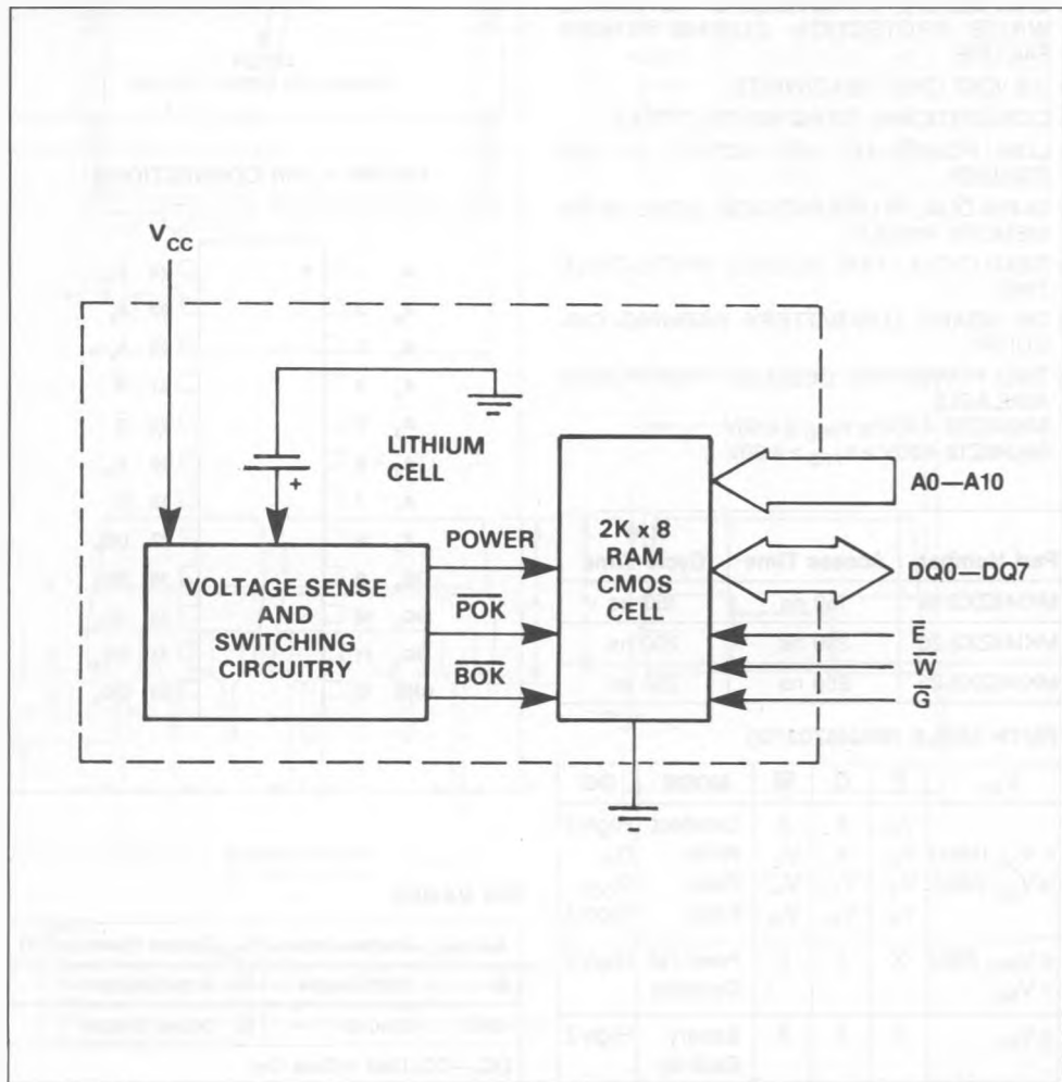
FIGURE 2. BLOCK DIAGRAM
