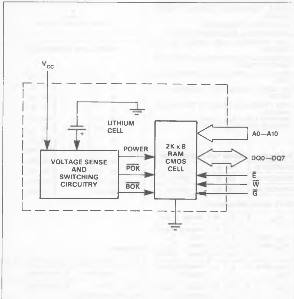
FIGURE 2. BLOCK DIAGRAM
