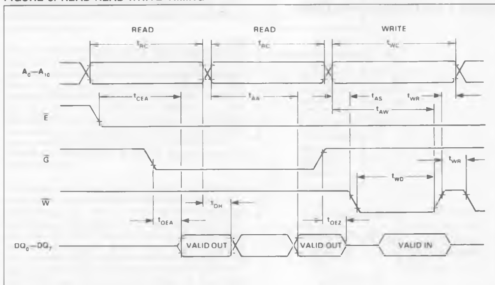
FIGURE 3. READ-READ-WRITE TIMING
