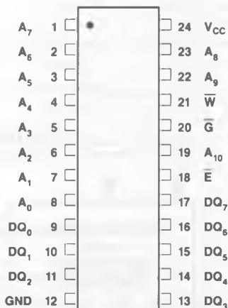
FIGURE 1. PIN CONNECTIONS
