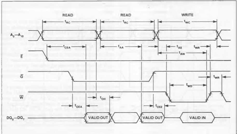
FIGURE 3. READ-READ-WRITE TIMING
