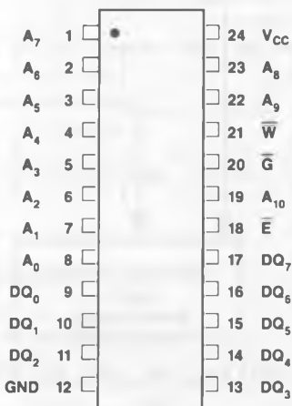
FIGURE 1. PIN CONNECTIONS
