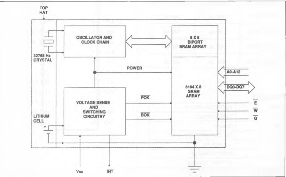
FIGURE 1. BLOCK DIAGRAM
