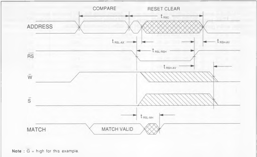
Figure 6 : Reset Timing.
