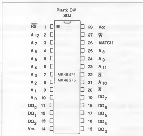
Figure 1 : Pin Connections.
