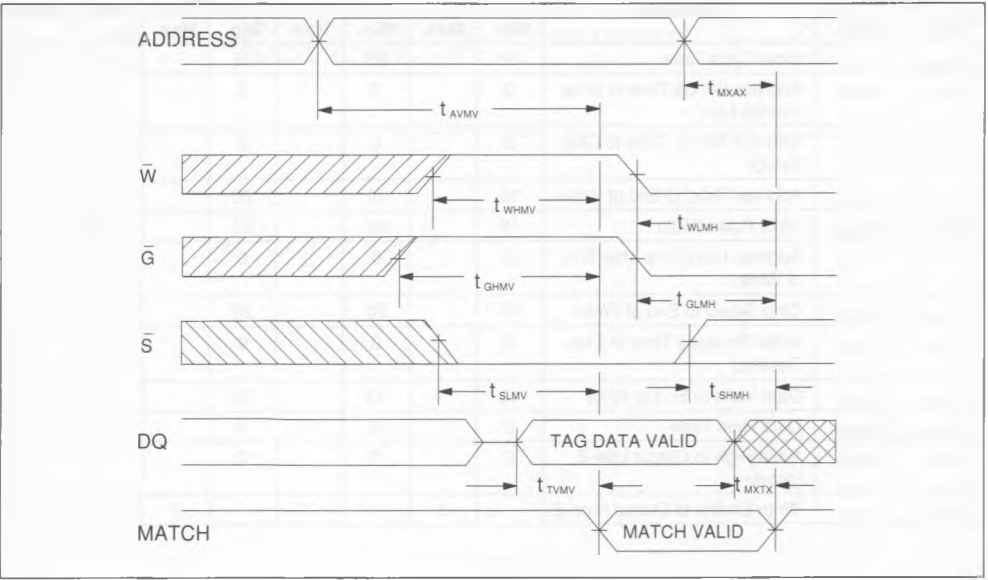
Figure 5 : Match Compare Timing.
