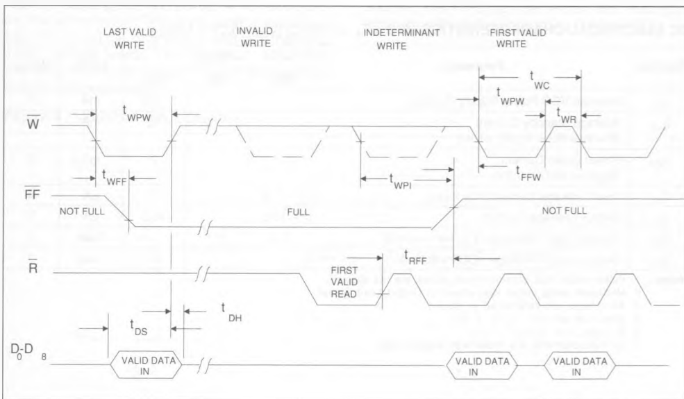
Figure 3A : Write and Full Flag Timing.
