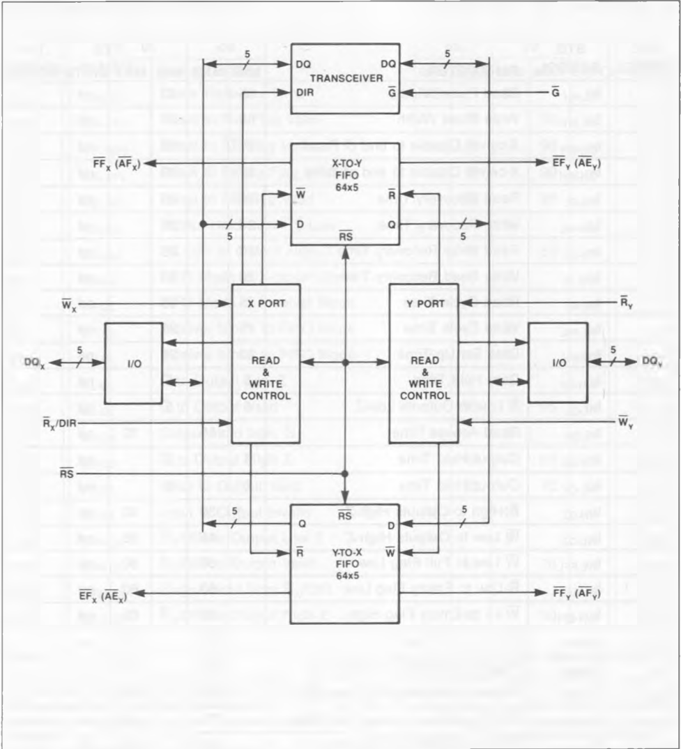
FIGURE 3. BLOCK DIAGRAM
