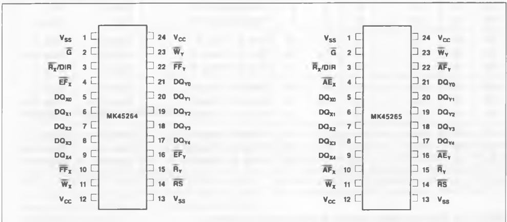
Figure 1 : Pin Connections.
