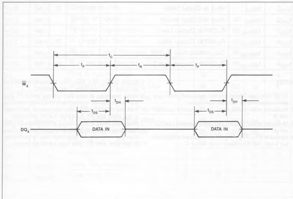
FIGURE 4. WRITE TIMING
