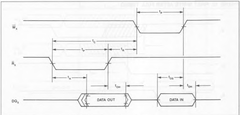
FIGURE 7. READ/WRITE TIMING
