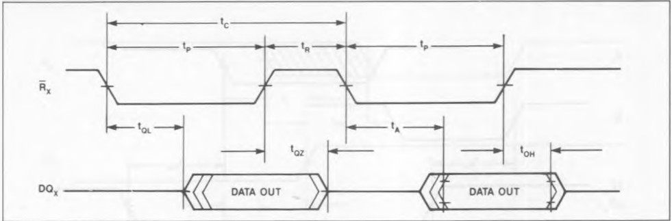
FIGURE 6. WRITE/READ TIMING
