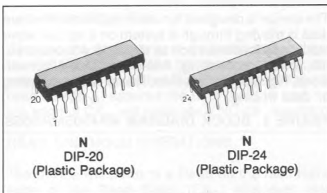
FIGURE 1. PIN CONFIGURATION
