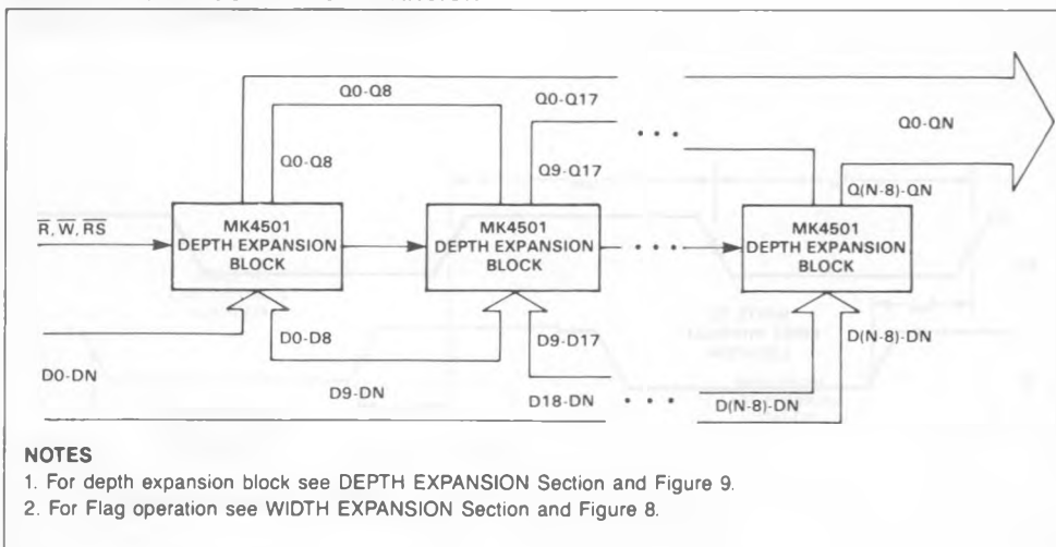
FIGURE 12. COMPOUND FIFO EXPANSION
