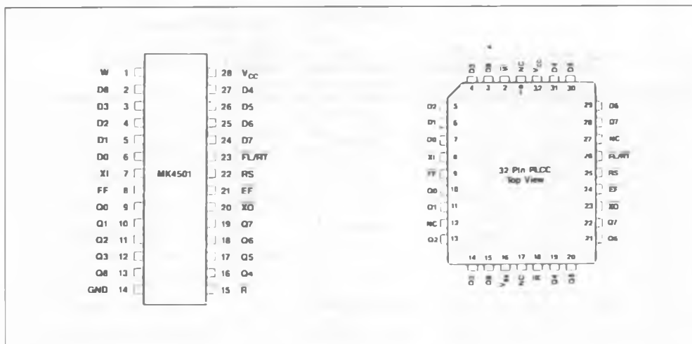
Figure 1 : Pin Connections.
