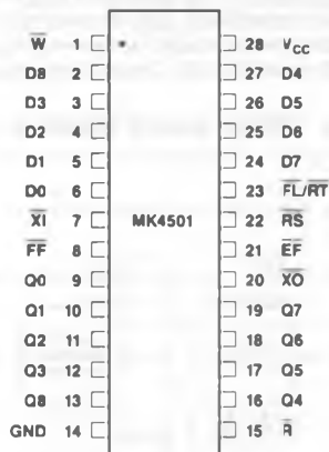
FIGURE 1. PIN CONNECTIONS
