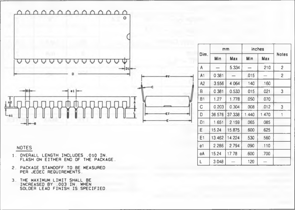
FIGURE 15. MK4501 PLASTIC (N TYPE) DUAL-IN-LINE, 28 PINS
