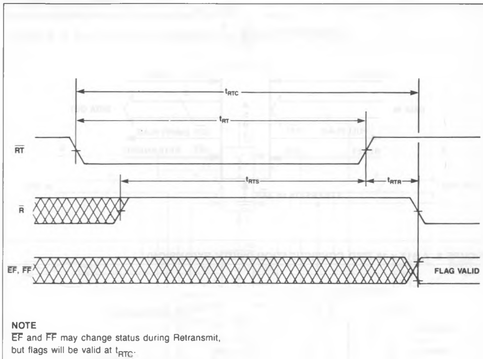
FIGURE 6. RETRANSMIT
