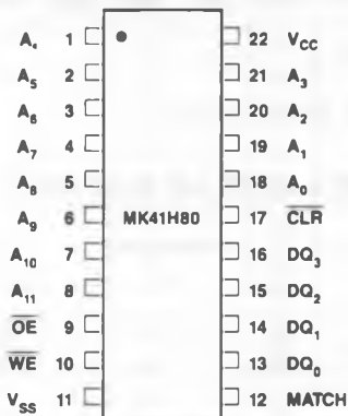
FIGURE 1. PIN CONNECTIONS
