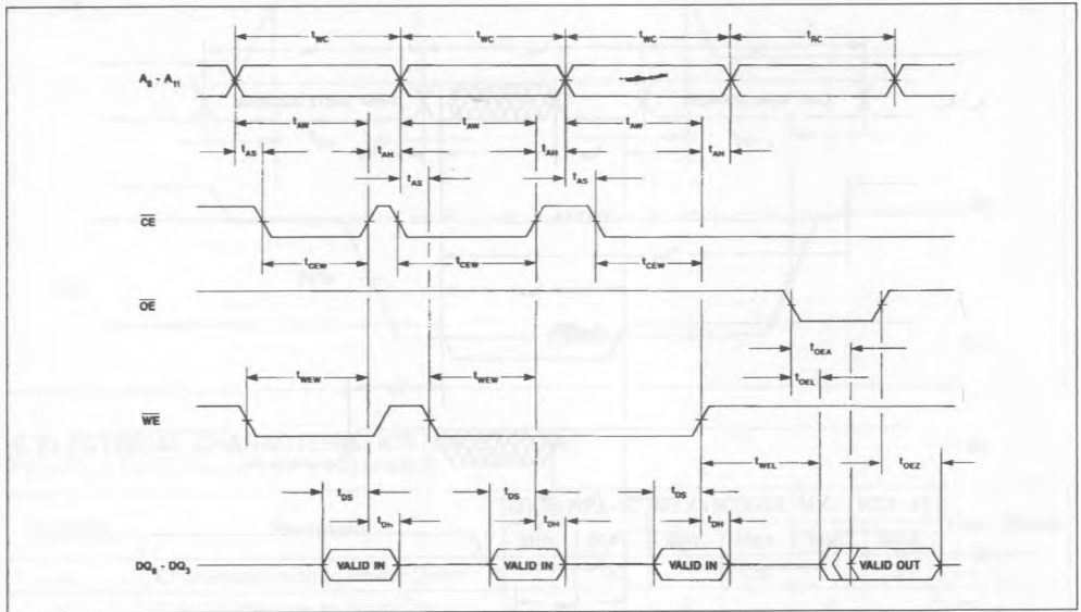
Figure 4 : Write–write–write–read Timing.
