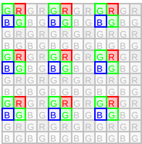
Figure 10. Bayer Space Sub-sampling Example
