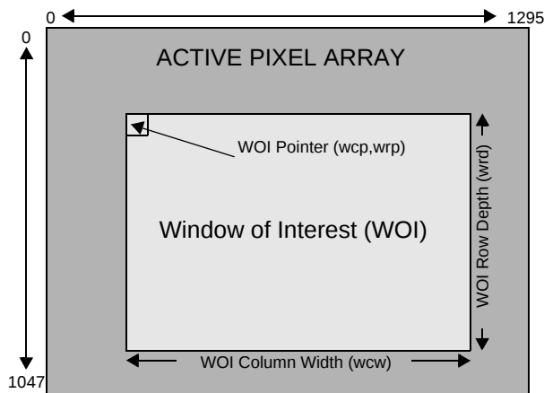
Figure 9. WOI Definition
