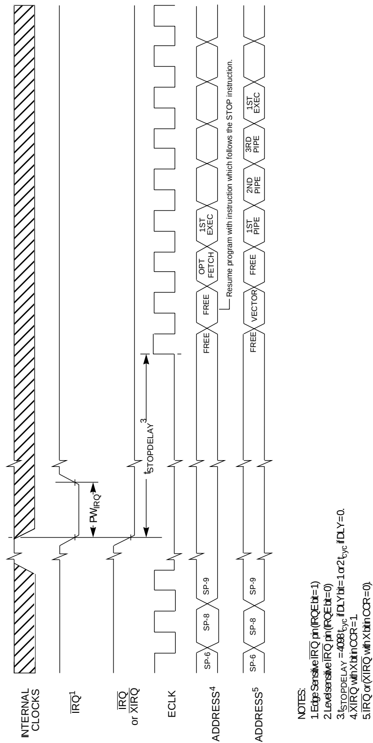
Figure 61 STOP Recovery Timing Diagram
