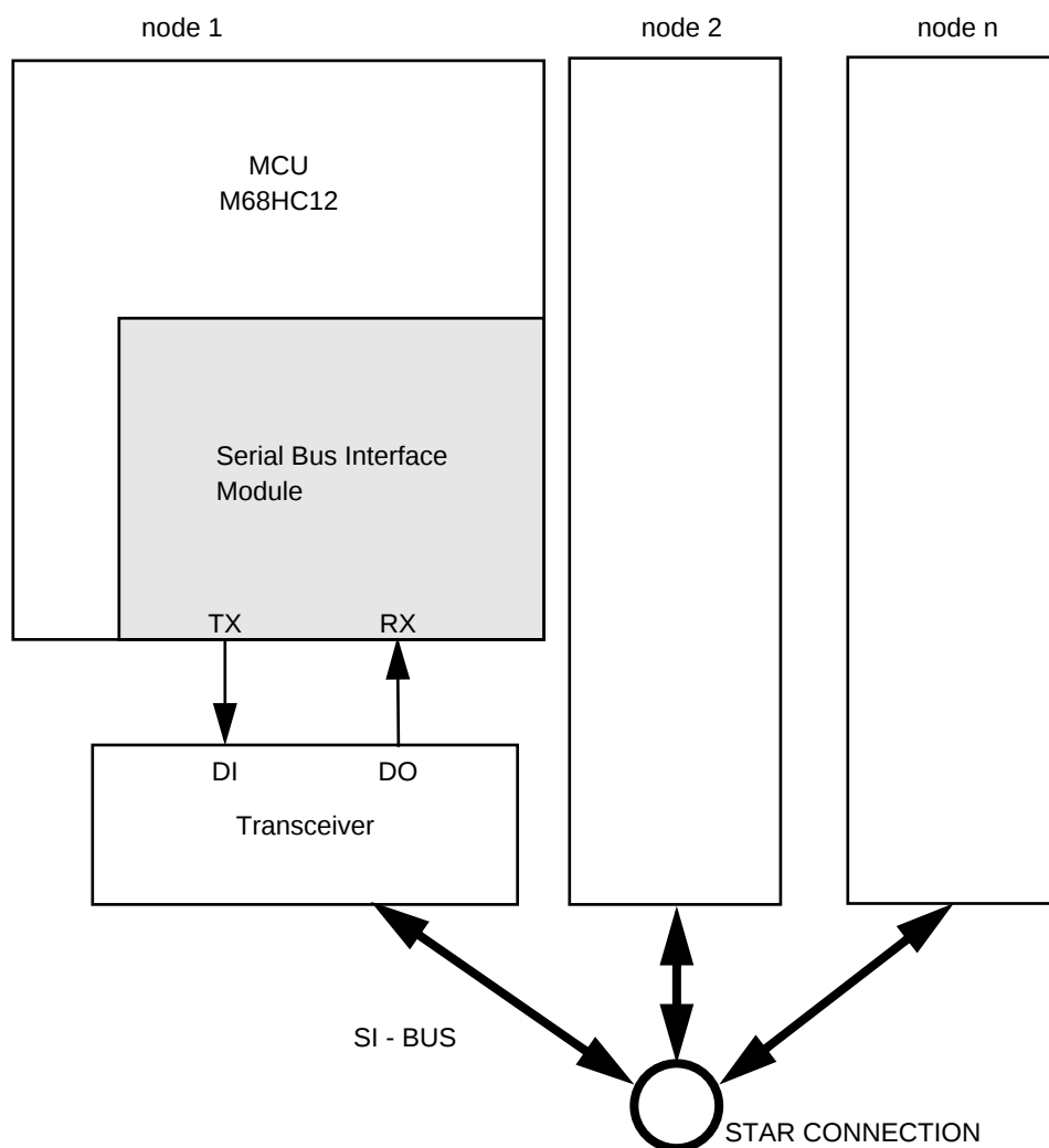
Figure 25 Byteflight™ System
