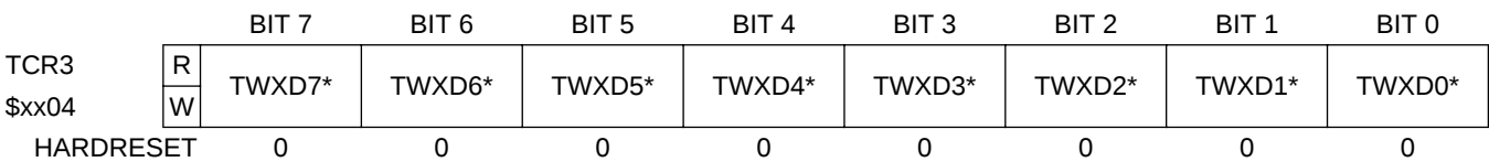
Figure 41 Time Configuration Register 3 (TCR3)
