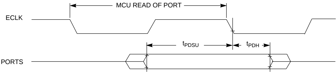
Figure 64 Port Read Timing Diagram
