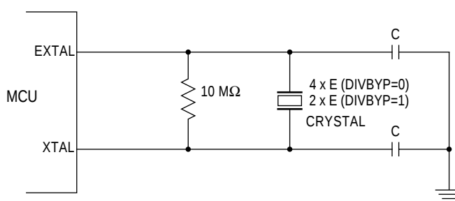
Figure 4 Common Crystal Connections
